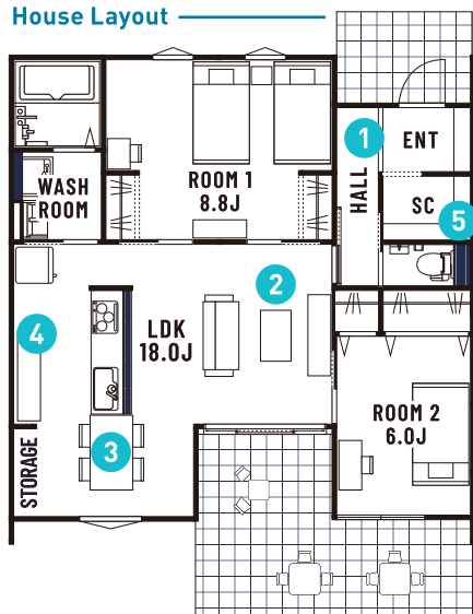
House Layout
